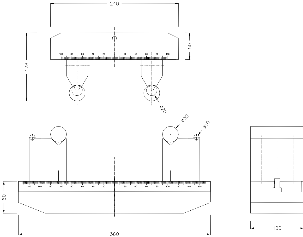
G22-11-360-4Pt Dimensions
